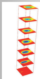
Temperature curve at various levels after the denitrification agent has been injected.
