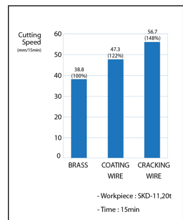
Comparison of Cutting Speed
