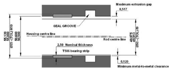
Gland for 50mm rod using 'standard' tolerances.
