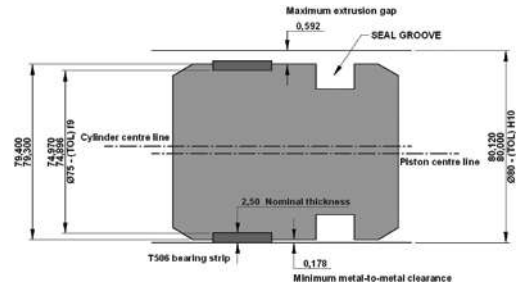
Piston for 80mm bore using 'standard' tolerances.
