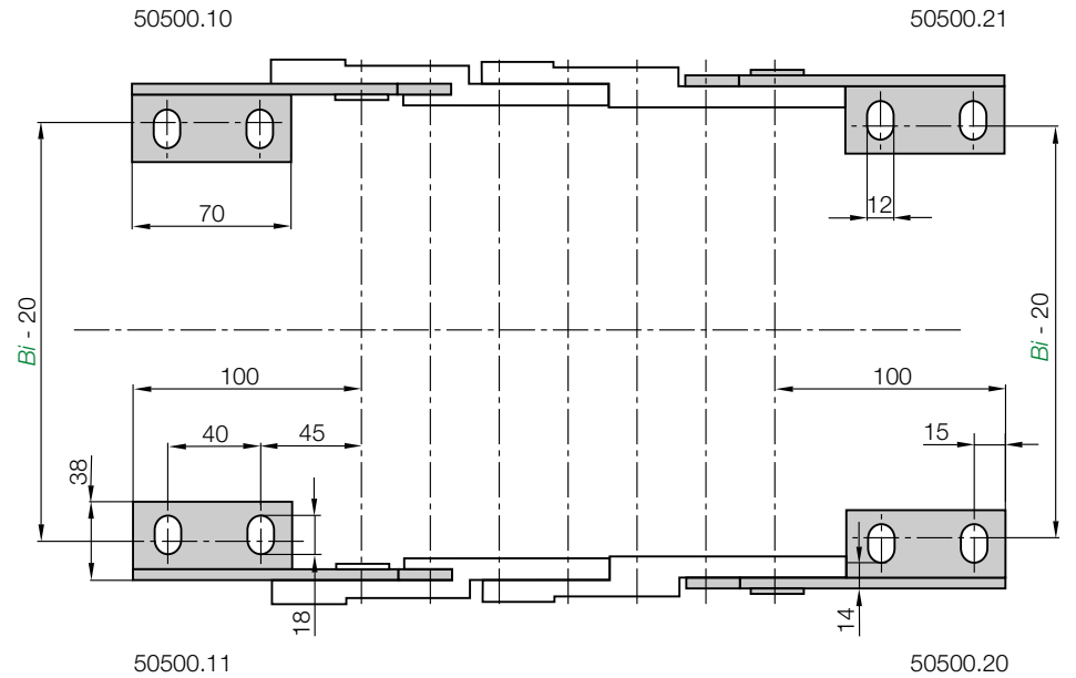
Moving end 50500.1
