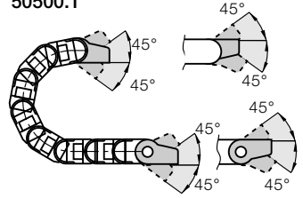
Fixed end 50500.2
