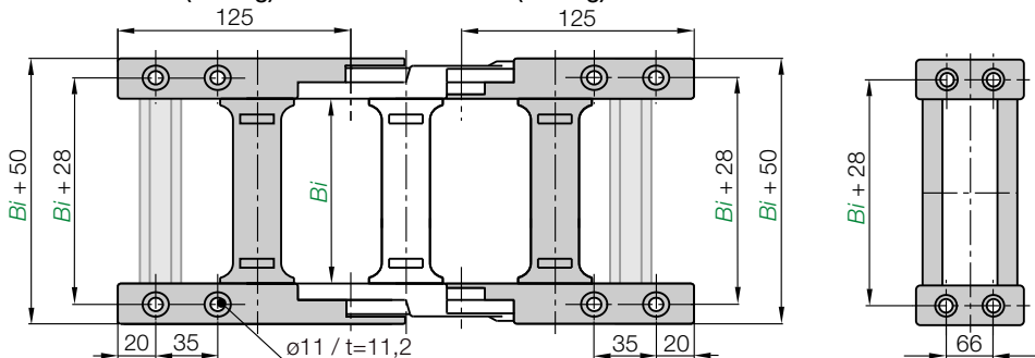
Fixed end 50500/98500...2 (pivoting) 51500/99500...2 (locking)
